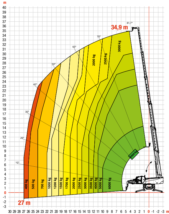
TR80.350
