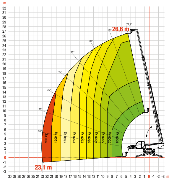
TR80.390
