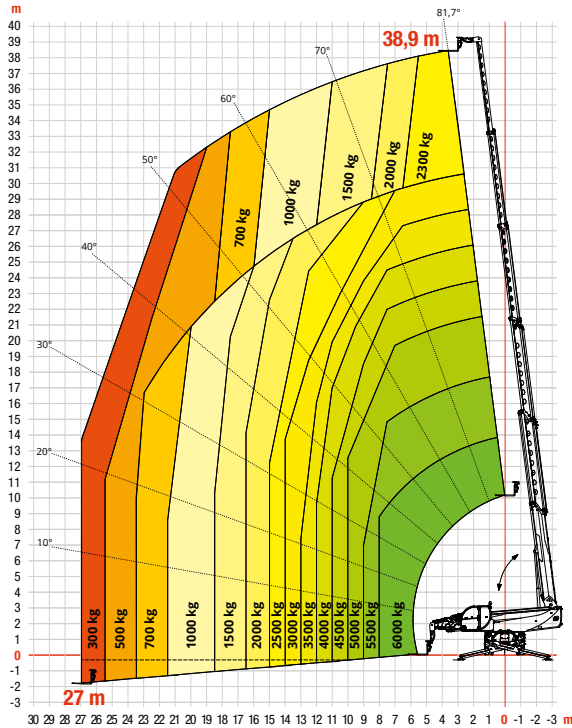
TR80.390
