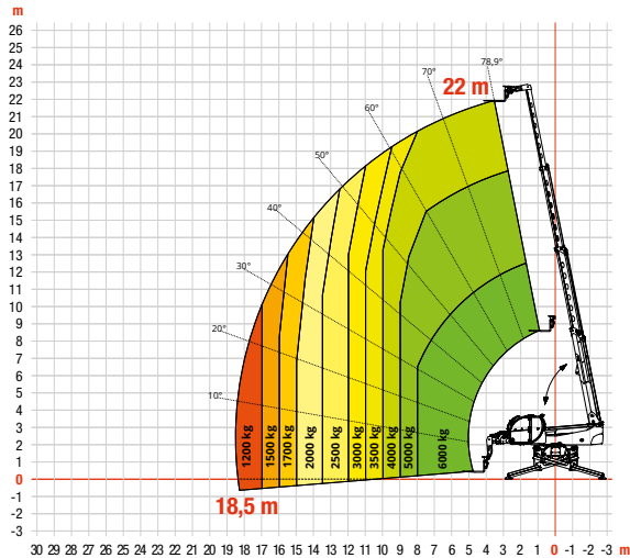
TR60.310
