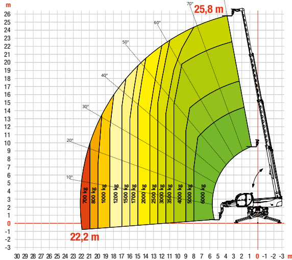
TR80.270
