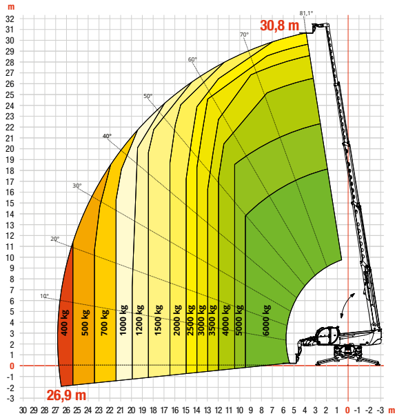
TR80.350
